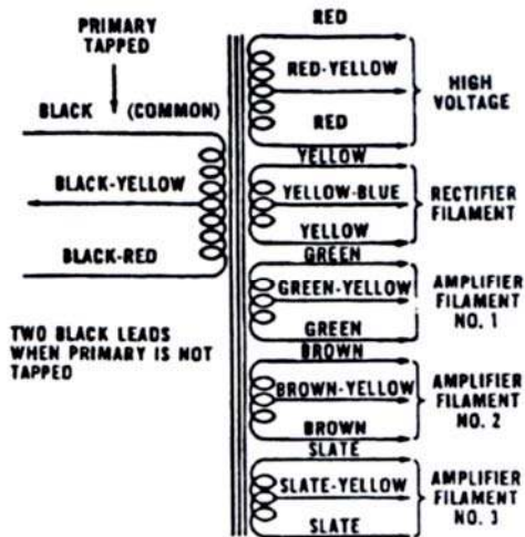
POWER TRANSFORMER
