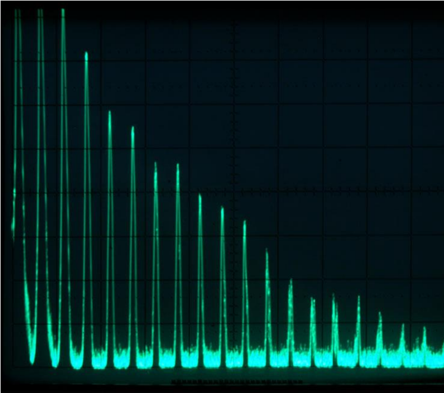
This is the crystal-only spectrum starting at 1 MHz with tapering harmonics (0 - 20 MHz span)
