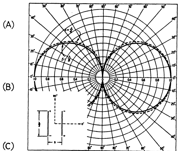
Fig. 4-22 — Free-space directive diagram of a two-element end-fire array with 180-degree phasing, in the plane containing the two parallel elements.
