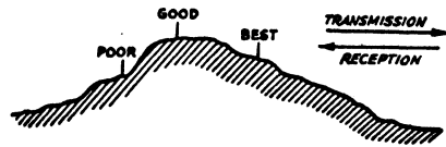
Fig. 1-7 — Propagation conditions are generally best when the antenna is located slightly below the top of a hill on the side that faces the distant station. Communication is poor when there is a sharp rise immediately in front of the antenna in the direction of communication.
