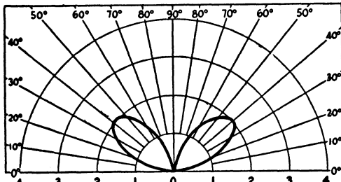
Fig. 2-56 — In direction of wire; height 1/2 wavelength.
