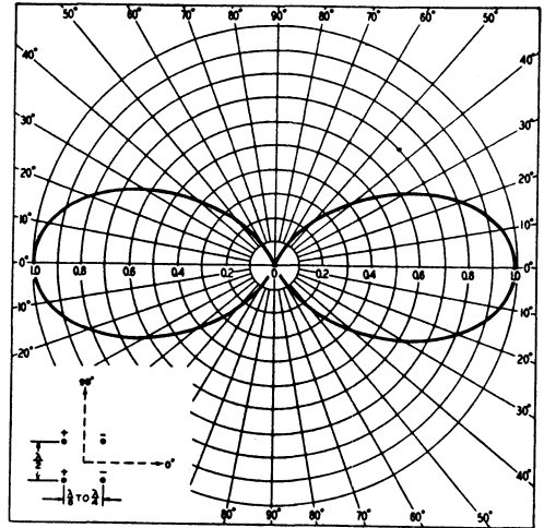
Fig. 16-9 — Free-space pattern of the four-element antenna shown in Fig. 16-8, in the plane perpendicular to the array axis. The pattern in the plane containing a set of end-fire elements is the same as Fig. 4-22 of Chapter Four.
