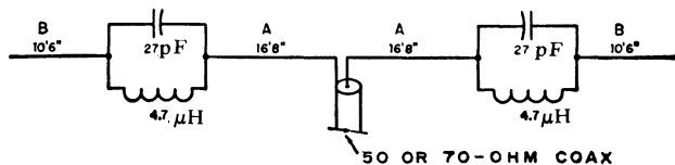
Fig. 6-16 — Sketch showing dimensions of a trap dipole covering the 40- through 10-meter bands (K2GU).
