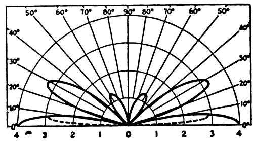
Fig. 2-69 — Height 1 wavelength.
