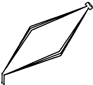
Fig. 5-17 — Three-wire rhombic antenna. Use of multiple wires improves the impedance characteristic of a nonresonant rhombic and increases the gain somewhat.
