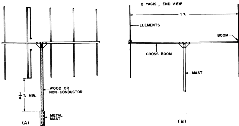
Fig. 11-43 — Methods of mounting Yagi antennas with the elements vertical. The boom-to-mast joint may be strengthened by a gusset plate. If the arrays are large enough to require diagonal bracing, such bracing should be of nonconducting material where it is close to the elements.
