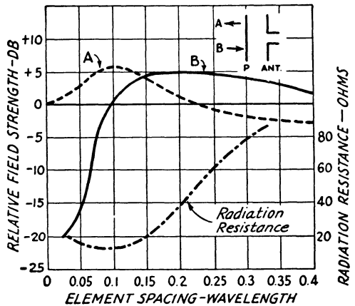
Fig. 4-37 — Theoretical gain of a two-element parasitic array over a half-wave dipole as a function of element spacing when the parasitic element is self-resonant.
