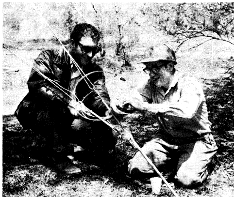
Fig. 14-12 — A guy cable is used to assure the turnbuckles remain in place after they are tightened. This procedure is an absolute requirement for a guyed tower system. (Photo by K1THQ)
