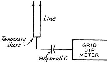
Fig. 3-54 — Using a grid-dip meter to check resonance of the antenna system for antenna currents on the transmission line. The small capacitance may be a short length of wire connected to the feed line, coupled lightly to the grid-dip-oscillator coil with a 1-turn loop.
