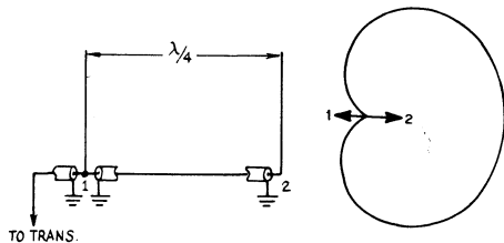
Fig. 8-7 — Pattern for two 1/4\text{-}\lambda verticals spaced 1/4 wavelength apart and fed 90 degrees out of phase. The arrow represents the axis of the elements, with the element on the right being the one of lagging phase.
