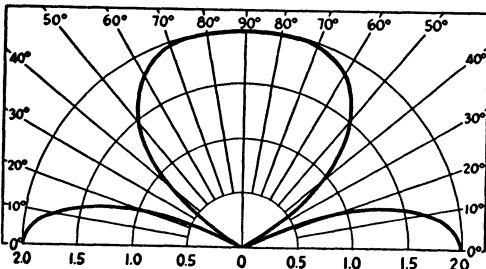
Fig. 2-38 – Vertical dipole antenna with center 1/2 wavelength high.
