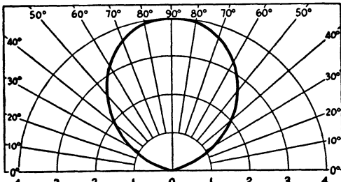
Fig. 2-54 — In direction of wire; height 1/4 wavelength.
