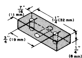
REXOLITE MOUNTING BLOCKS
