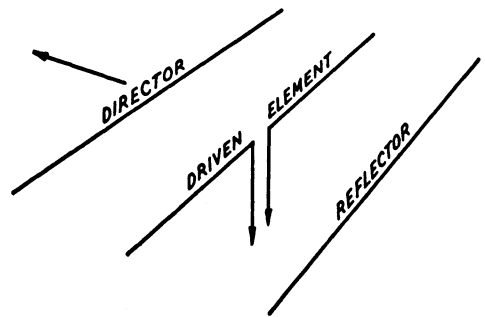
Fig. 4-40 — Antenna system using a driven element and two parasitic elements, one as a reflector and one as a director.
