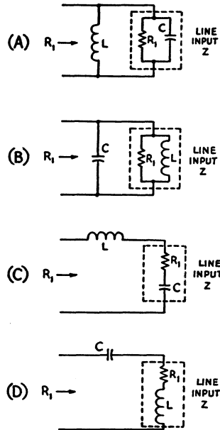
Fig. 3-39 – Compensating for reactance present in the line input impedance.
