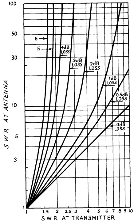
Fig. 3-24 – SWR at input end of transmission line vs. SWR at load end for various values of matched-line loss.
