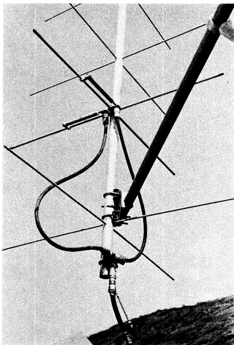
Fig. 12-1 — This vhf crossed Yagi antenna design by KH6IJ was presented in January 1973 QST . Placement of the phasing harness and T connector is shown in the lower half of the photograph. Note that the gamma match is mounted somewhat off of element center for better balance of rf voltages on elements.
