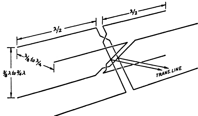
Fig. 16-11 — Eight-element driven array combining collinear and parallel elements for broadside and end-fire directivity.
