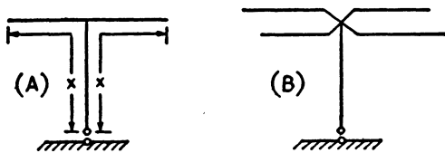
Fig. 2-77 — Simple top loading of a vertical antenna. The antenna terminals, indicated by the small circles, are the base of the antenna and ground, and should not be taken to include the length of any lead-ins or connecting wires.
