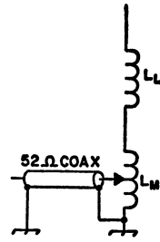
Fig. 15-9 — A method of matching the loaded whip to 52-ohm coax cable. L_L is the loading coil and L_M the matching coil.
