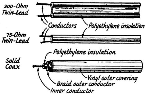
Fig. 3-33 — Construction of parallel-conductor and coaxial lines with solid dielectric.
