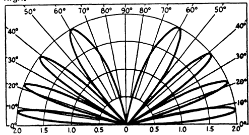
Fig. 2-35 — Horizontal antennas 2 wavelengths high.
