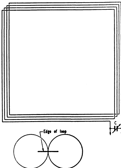
Fig. 16-1 — Small loop, consisting of several turns of wire having a total length very much less than a wavelength. The directional pattern of such a loop is as shown in the small drawing, with maximum response in the plane of the loop.
