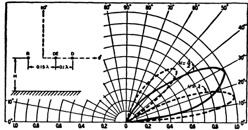
Fig. 4-48 — Vertical patterns of the antenna of Fig. 4-47 in the vertical plane at right angles to the direction of the antenna elements.
