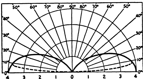
Fig. 2-66 — Height 1/4 wavelength.
