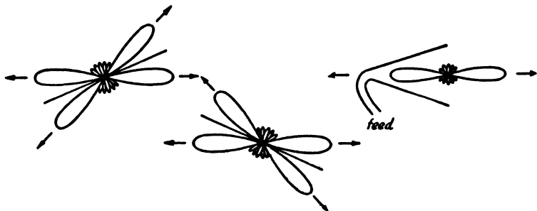
Fig. 5-6 — Two long wires and their respective patterns are shown at the left. If these two wires are combined to form a V whose apex angle is twice that of the major lobes of the wires and the wires are excited out of phase, the radiation along the bisector of the V adds and the radiation in the other directions tends to cancel.
