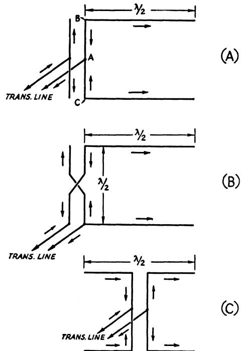
Fig. 4-17 — Two-element broadside arrays, showing different methods of supplying power.
