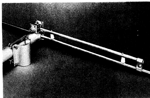
Fig. 11-15 — Typical gamma-match construction. The variable capacitor, 50 pF, should be mounted in an inverted plastic cup or other device to protect it from the weather. The gamma arm is about 12 inches long for 50 MHz, 5 inches for 144 MHz.
