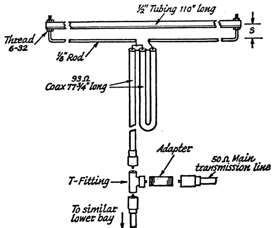
Fig. 11-25 — Details of the driven elements and phasing system used in the 50-MHz stacked array. The folded dipole is set up so that its feed impedance is approximately 400 ohms. Two half-wave baluns and half-wave phasing sections step down to about 100 ohms. The two bays thus connected in parallel may be fed with 50-ohm coax directly.
