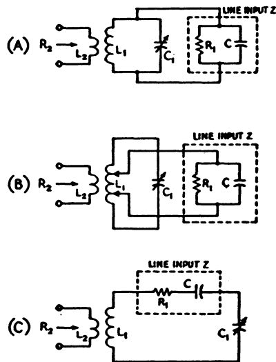
Fig. 3-38 - Line input impedances containing both resistance and reactance can be represented as shown enclosed in dotted lines, for capacitive reactance. If the reactance is inductive, a coil is substituted for the capacitance C.
