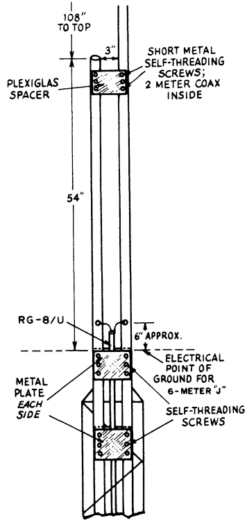
Fig. 11-47 - Details of the 6-meter J pole.
