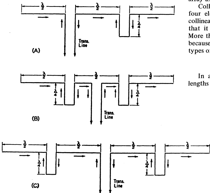
Fig. 4-12 — Three- and four-element collinear arrays. Alternative methods of feeding a three-element array are shown at A and B. These drawings also show the current distribution on the antenna elements and phasing stubs. A matched transmission line can be substituted for the tuned line by using a suitable matching section.
