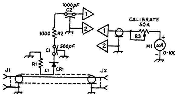
Fig. 17-12 — Circuit diagram for the line sampler. C1 — 500-pF feedthrough capacitor, solder-in type. C2 — 1000-pF feedthrough capacitor, threaded type.
