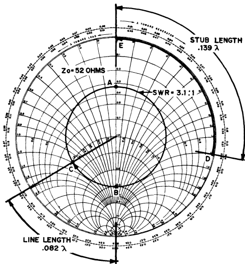
Fig. 3-77 — Smith Chart method of determining the dimensions for stub matching.
