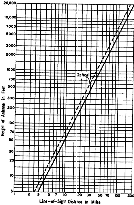
Fig. 1-6 — Distance to the horizon from an antenna of given height. The solid curve includes the effect of atmospheric refraction. The optical line-of-sight distance is given by the broken curve.
