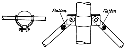
Fig. 11-21 — Method of mounting suspension braces to a pipe mast is shown at the right. The braces are flattened at the ends and bolted to semicircular clamps formed from aluminum sheet. A method of mounting elements on a boom is shown at the left. Elements go through holes drilled through the boom, and are held tight by the pull-down clamps as shown. The clamps can be made from sheet aluminum.
