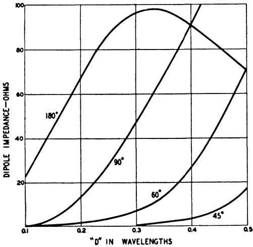
Fig. 11-37 — Feed impedance of the driven element in a corner-reflector array, for various corner angles of 180 (flat sheet), 90, 60 and 45 degrees.
