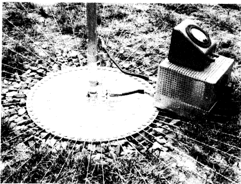
Fig. 10-7 — Base of the vertical antenna showing the 60 radials. The aluminum disk is 15 inches in diameter and 1/4-inch thick. Sixty tapped holes for 1/4-20 aluminum hex-head bolts form the outer ring and 20 form the inner ring. The insulator is polystyrene material (phenolic or Plexiglas suitable) with a one-inch diameter. Also shown is the impedance bridge used for measuring input resistance.
