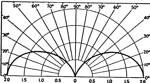
Fig. 2-36 – Vertical dipole antenna with center 1/4 wavelength high.
