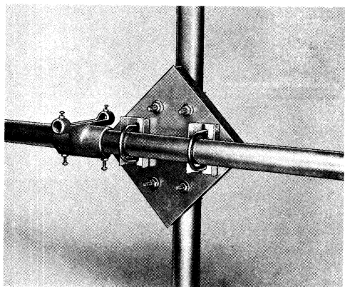
Fig. 11-16 — Closeup photograph of the boom mounting for the 3-element 50 MHz array. A sheet of aluminum 6 inches square is backed up by a piece of wood of the same size. TV-type U clamps hold the boom and vertical support together at right angles. At the left of the mounting assembly is one of the aluminum castings for holding the beam elements.
