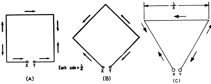
Fig. 2-84 — At A and B, loops having sides 1/4 wavelength long, and at C having sides 1/3 wavelength long (total conductor length one wavelength). The polarization depends on the orientation of the loop and the point at which the terminals X-Y are located.
