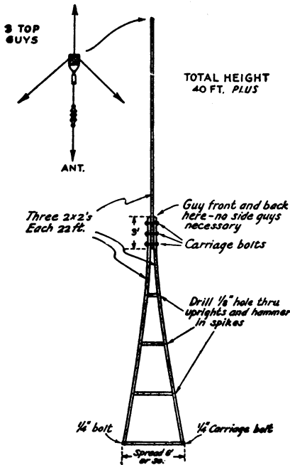
Fig. 13-23 — The "A-frame" mast, lightweight and easily constructed and erected.
