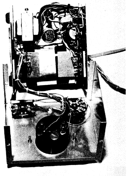
Fig. 14-7 — Inside view of the Hy-Gain control box.
