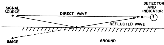
Fig. 17-21 — On an antenna test range, energy reaching the receiving equipment may arrive after being reflected from the surface of the ground, as well as by the direct path. The two waves may tend to cancel each other, or may reinforce one another, depending on their phase relationship at the receiving point.
