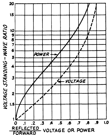
Fig. 17-7 — Chart for finding voltage standing-wave ratio when the ratio of reflected-to-forward voltage or reflected-to-forward power is known.
