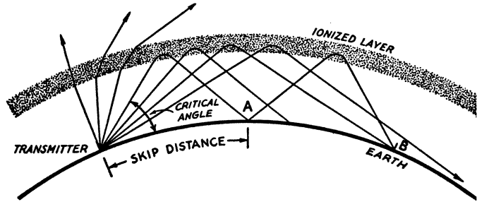
Fig. 1-8 — Behavior of waves on encountering the ionosphere. Waves entering the ionized region at angles higher than the critical angle are not bent enough to be returned to earth. Waves entering at angles below the critical angle reach the earth at increasingly greater distances as the angle approaches the horizontal.
