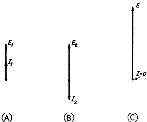
Fig. 3-9 — Voltage and current at the end of an open-circuited line. A — outgoing voltage and current; B — reflected voltage and current; C — resultant.
