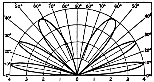
Fig. 2-65 — At right angles to wire; height 1-1/2 wavelength.
