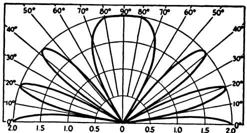
Fig. 2-41 – Vertical dipole antenna with center 1-1/2 wavelengths high.
