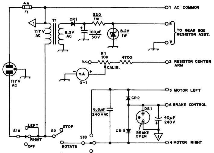
Fig. 14-6 — Circuit diagram for the Hy-Gain rotor control box. The 6.8- \mu F, 240-V ac capacitor is taken from the original Hy-Gain control head. CR1, CR2 and CR3 are conventional power diodes, 1000 PRV at 1 A. T1 is rated for one ampere. R1 is a linear-taper composition two-watt control. The indicator meter shown in the photographs is a model 524, manufactured by Simpson Electric. S2 is a spring-return type.
