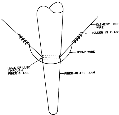
Fig. 9-11 — A method of assembling a corner of the wire loop of a quad element to the spreader arm.
