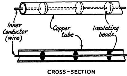
Fig. 3-31 — Construction of air-insulated coaxial lines.
