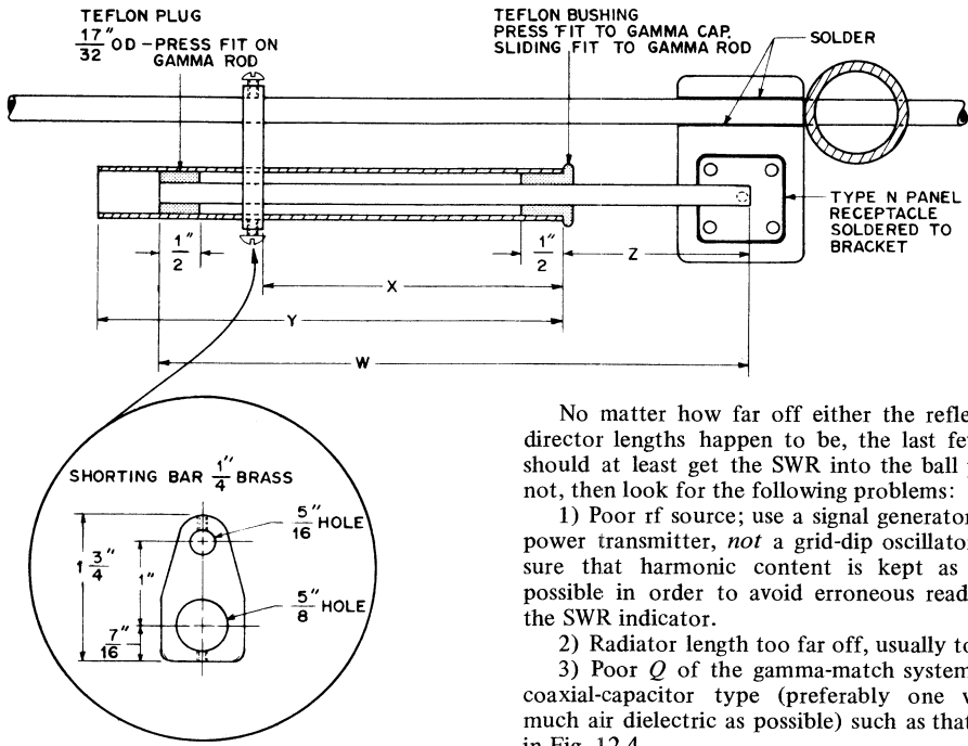
Fig. 12-4 – Gamma-match construction details.
