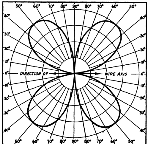
Fig. 2-16 — Free-space directive diagram of a 1-wavelength harmonic antenna in the plane containing the wire axis.
