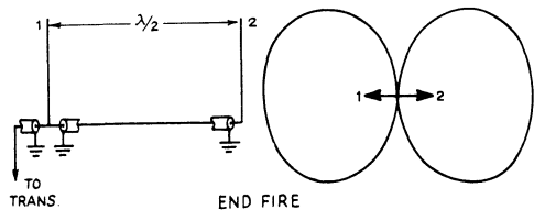
Fig. 8-6 — Pattern for two 1/4\lambda verticals spaced one-half wavelength apart fed 180 degrees out of phase. The arrow represents the axis of the elements.
