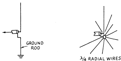
Fig. 8-8 — An 8\text{-} to 10\text{-} ft. ground rod may provide a satisfactory ground system in marshy or beach areas, but in most locations a system of radial wires will be necessary.
