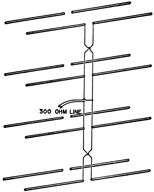
Fig. 11-33 — Schematic drawing of a 16-element array. A variable Q section may be inserted at the feed point if accurate matching is desired. Reflector spacing is 0.2 wavelength.
