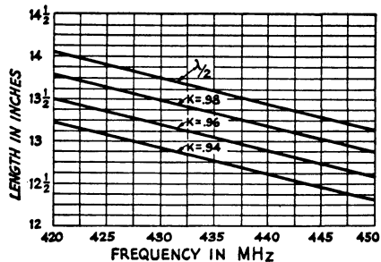
Fig. 11-1 — Frequency vs. length in inches for the 50-, 144-, 220- and 420-MHz bands, for a free-space half wavelength and resonant antenna lengths for various element length/thickness ratios (see Chapter Two). Lengths for values of K other than those given can be found by linear interpolation, e.g., the curve for K = 0.97 lies midway between the curves for K = 0.96 and 0.98, etc. To find the free-space wavelength used in calculating spacings multiply the length given for λ/2 by 2.
