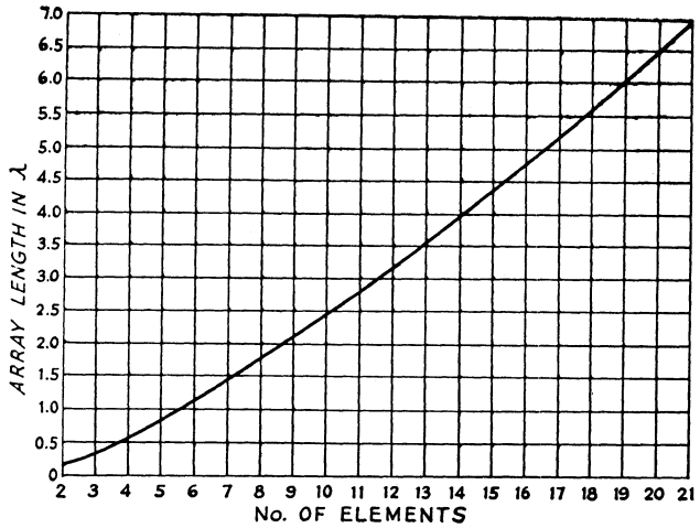
Fig. 4-51 — Optimum length of Yagi antenna as a function of number of elements.
