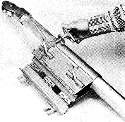
Fig. 14-8 — A gin pole is a mechanical device which can be clamped to a tower leg to aid in the assembly of sections as well as the installation of antennas. The aluminum tubing extends through the clamp and may be slipped into position before the tubing clamp is tightened. A rope should be routed through the tubing and over the pulley mounted at the top. See Fig. 14-9 for installation details.
