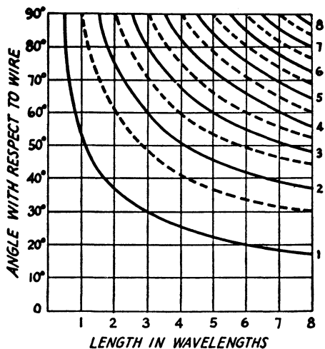
Fig. 5-2 — Angles at which radiation from long wires is maximum (solid curves) and zero (broken curves). The major lobe, No. 1, has the power gains given by Fig. 5-1. Secondary lobes have smaller amplitude, but the maxima may exceed the radiation intensity from a half-wave dipole.
