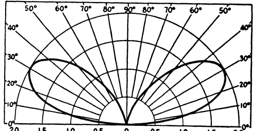
Fig. 2-27 — Horizontal antennas 1/2 wavelength high.
