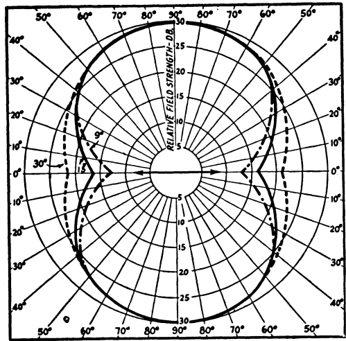
Fig. 2-46 — Directive patterns of a horizontal half-wave antenna at three radiation angles, 9, 15 (solid line), and 30 degrees. The direction of the antenna itself is shown by the arrow. These patterns are plotted to a 30-dB scale, which is about proportional to signal strength as determined by ear. If 30 dB represents an S-9 signal, 0 on the scale will be about S-3. All three patterns are plotted to the same maximum, but the actual amplitudes at the various angles will depend upon the antenna height, as described in the text. The patterns shown here indicate only the shape of the directive diagram as the angle is varied.
