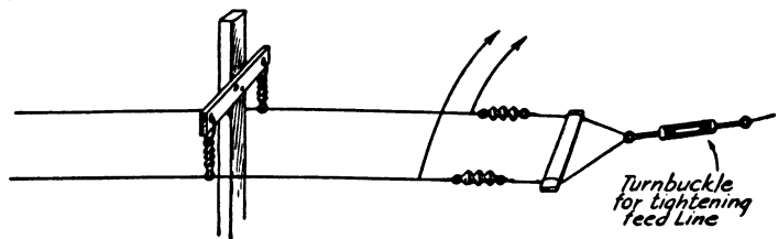
Fig. 13-11 — A support for open-wire line. The support at the antenna end of the line must be sufficiently rigid to stand the tension of the line.
