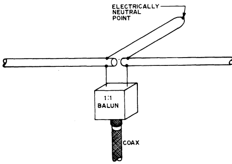
Fig. 3-69 — The hairpin match.
