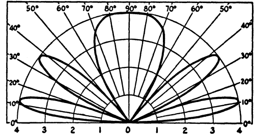
Fig. 2-63 — At right angles to wire; height 1-1/4 wavelength.
