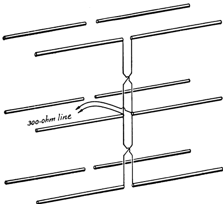
Fig. 11-29 — Element arrangement and feed system of the 12-element curtain array. Reflectors are spaced 0.15 wavelength behind the driven elements.
