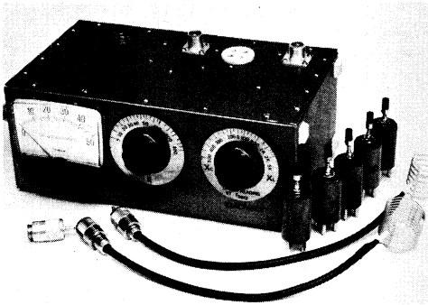
Fig. 17-16 — An RCL bridge for measuring unknown values of complex impedances. A plug-in coil is used for each frequency band. The bridge operates at an rf input level of about 5 volts; pickup-link assemblies for use with a grid-dip oscillator are shown. Before measurements are made, the bridge must be balanced with a non-reactive load connected at its measurement terminals. This load consists of a resistor mounted inside a coaxial plug, shown in front of the instrument at the left. The aluminum box measures 4-1/4 × 10-3/4 × 6-1/8 inches and is fitted with a carrying handle on the left end and self-sticking rubber feet on the right end and bottom. Dials are Millen No. 10009 with skirts reversed and calibrations added.
