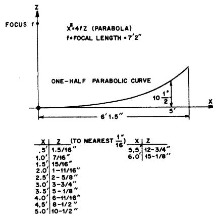
Fig. 12-16 — Parabolic template for 12-foot, 3-inch dish.
