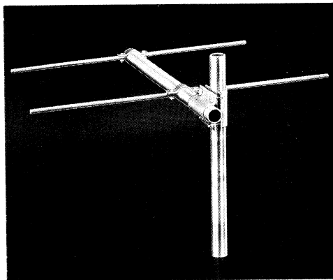
Fig. 11-30 — Model showing the method of assembly for all-metal construction of phased arrays. Dimensions of clamps are given in Fig. 11-31.
