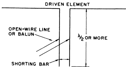
Fig. 11-8 — Combination tuning and matching stub for vhf arrays. The sliding shorting bar is used for tuning the driven element along with the stub itself. The transmission line (or balun, if coax line is used) is moved along the stub until the point at which the SWR is closest to unity is found.
