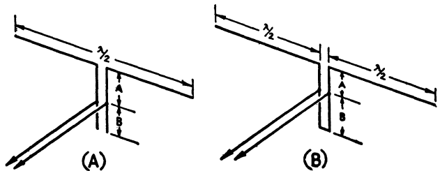
Fig. 3-76 — Application of matching sections to common antenna types.
