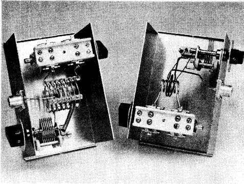
Fig. 11-12 — Practical construction of matching circuits of the type shown in Fig. 11-11, for 50 MHz, left, and 144 MHz, right. Each is built on one piece of a two-piece aluminum box. These views are of the inside of the top piece.
