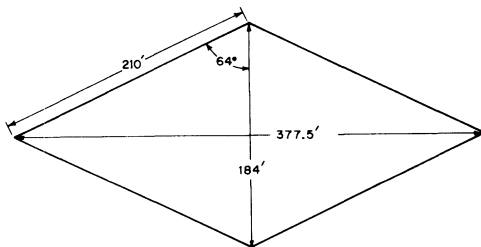
Fig. 5-15 — Rhombic antenna dimensions for a compromise design between 20- and 10-meter requirements, as discussed in the text. The leg length is 6 λ on 10 meters, 3 λ on 20.
