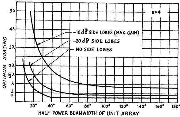
Fig. 4-55 — Optimum stacking spacing for four-unit arrays.
