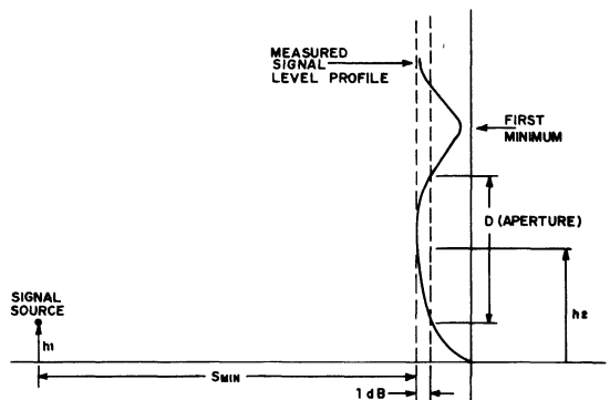
Fig. 17-23 — Sample plot of a measured vertical profile.
