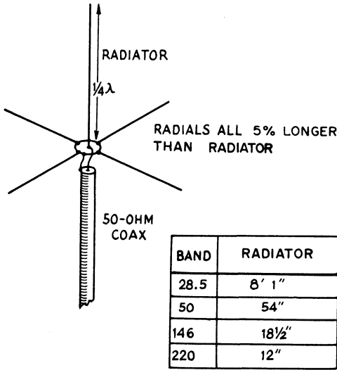
Fig. 11-44 — The simple 1/4-wavelength ground plane.
