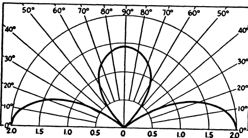
Fig. 2-37 – Vertical dipole antenna with center 3/8 wavelength high.
