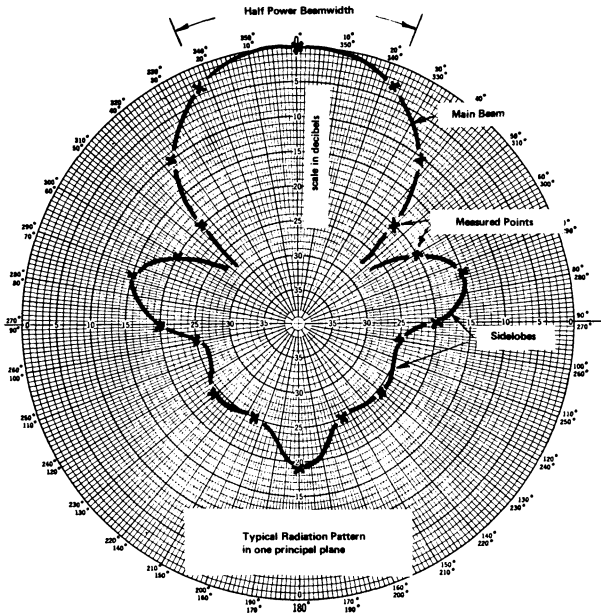
Fig. 17-25 – Sample plot of a measured radiation pattern, using techniques described in the text.
