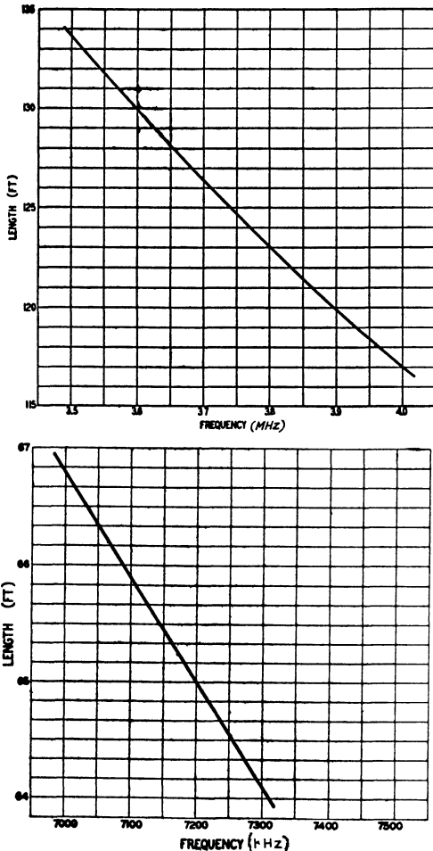
Fig. 8-2 — The above charts can be used to determine the length of a half-wave antenna of wire.
