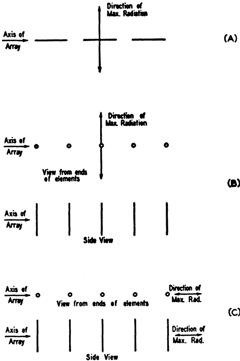
Fig. 4-3 — Representative broadside arrays are shown at A and B, the first with collinear elements, the second with parallel elements. An end-fire array is shown at C. Practical arrays may combine both broadside and end-fire directivity, including both parallel and collinear elements.
