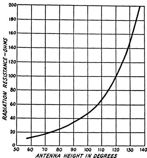
Fig. 2-74 — Radiation resistance vs. free-space antenna height in electrical degrees for a vertical antenna over perfectly conducting ground, or over a highly conducting ground plane. This curve also may be used for center-fed antennas (in free space) by multiplying the radiation resistance by two; the height in this case is half the actual antenna length.
