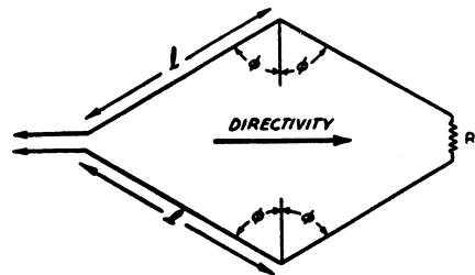
Fig. 5-12 — The nonresonant rhombic antenna.
