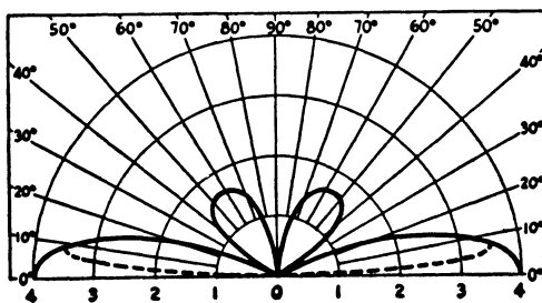
Fig. 2-67 — Height 1/2 wavelength.
