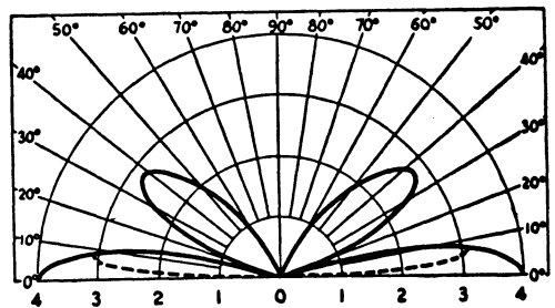
Fig. 2-68 — Height 3/4 wavelength.
