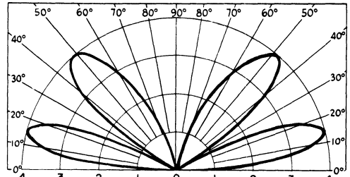
Fig. 2-61 — At right angles to wire; height 1 wavelength.
