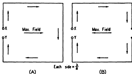
Fig. 2-82 — Half-wave loops, consisting of a single turn having a total length of 1/2 wavelength.
