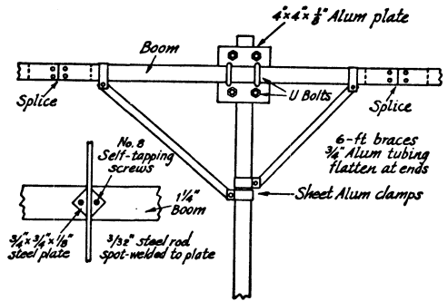
Fig. 11-28 — Boom support and element mounting used in the 13-element Yagi antenna of Fig. 11-27.
