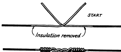
Fig. 13-3 — Correct method of splicing antenna wire.
