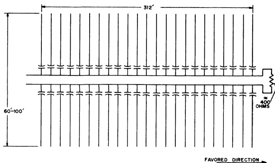
Fig. 16-4 — The fishbone antenna provides higher gain per acre than does a rhombic. It is essentially a wave antenna which evolved from the Beverage antenna.
