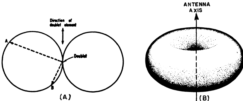
Fig. 2-12 — At A, directive diagram of an elementary doublet in the plane containing the wire axis. The length of each dash-line arrow represents the relative field strength in that direction. At B, the solid pattern of the same antenna. These same diagrams apply to any antenna considerably less than a half wavelength long.
