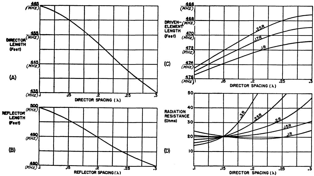
Fig. 9-5 — Element lengths for 3-element Yagis. These lengths will hold closely for tubing elements supported at or near the center. The radiation resistance (D) is useful information in planning for a matching system, but it is subject to variation with height above ground and must be considered an approximation. The driven-element length (C) may require modification for tuning out reactance if a gamma- or hairpin-match feed system is used.
