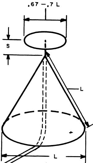
Fig. 16-13 - The discone antenna is a wideband, coaxially fed type best suited to vhf and uhf coverage because of its cumbersome size at hf. Dimension L is equal to a free-space quarter wavelength at the lowest operating frequency. The profile of the skirt is an equilateral triangle; the skirt itself can be of a cage type of construction, with adjoining wires separated by not more than .02\lambda at the bottom of the cone. Dimension S varies from 1 to 6 inches, depending on the low-frequency cutoff of the design.
