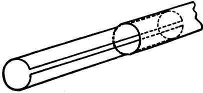
Fig. 11-2 — A simple method of providing for adjustment of element lengths. The insert is made of the same size tubing as the element, but is slotted and compressed to permit insertion into the ends of the elements.
