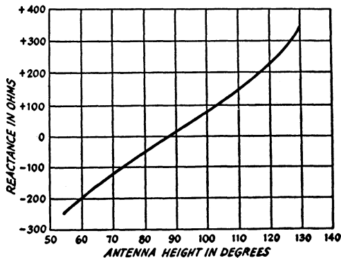
Fig. 2-76 — Approximate reactance of a vertical antenna over perfectly conducting ground and having a length/diameter ratio of about 1000. Actual values will vary considerably with length/diameter ratio. The remarks under Fig. 2-74 also apply to this curve.
