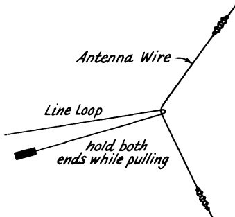
Fig. 13-20 — A weighted line thrown over the antenna can be used to pull the antenna to one side to avoid overhanging obstructions, such as branches of trees in the path of the antenna, as the antenna is pulled up. When the obstruction has been cleared, the line can be removed by releasing one end.
