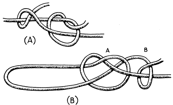
Fig. 13-7 — This is one type of knot that will hold with smooth rope, such as nylon. A shows the knot for splicing two ends. B shows the use of a similar knot in forming a loop, as might be needed for attaching an insulator to a halyard. Knot A is first formed loosely 10 or 12 inches from the end of the rope; then the end is passed through the eye of the insulator and knot A. Knot B is then formed and both knots pulled tight. (K7HDB.)
