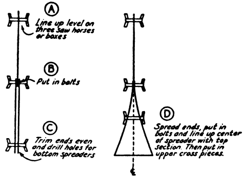
Fig. 13-24 — Method of assembling the "A-frame" mast.
