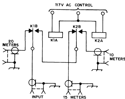
Fig. 9-14 — Suitable circuit for relay switching of bands for the three-band quad. A 3-wire control cable is required. K1, K2 — Any type of relay suitable for rf switching, coaxial type not required (Potter and Brumfeld MR11A acceptable; although this type has double-pole contacts, mechanical arrangements of most single-pole relays make them unacceptable for switching of rf).
