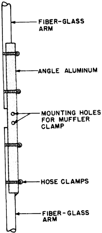
Fig. 9-10 — Details of one of two assemblies for a spreader frame. The two assemblies are joined to form an X with a muffler clamp mounted at the position shown.
