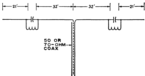
Fig. 6-15 — Layout of multiband antenna using traps constructed as shown in Fig. 6-14. The capacitors are 100 pF each, transmitting type, 5000-volt dc rating (Centralab 850SL-100N). Coils are 9 turns No. 12, 2-1/2 inch diameter, 6 turns per inch (B&W 3029) with end turns spread as necessary to resonate the traps to 7200 kHz. These traps, with the wire dimensions shown, resonate the antenna at approximately the following frequencies on each band: 3900, 7250, 14,100, 21,500 and 29,900 kHz (based on measurements by W9YJH).
