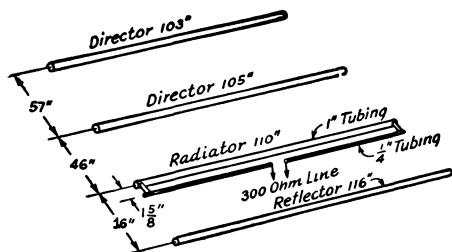
Fig. 11-17 — Dimensional drawing of the 4-element 50-MHz array. Element lengths and spacings were derived experimentally for maximum forward gain at 50.5 MHz.
