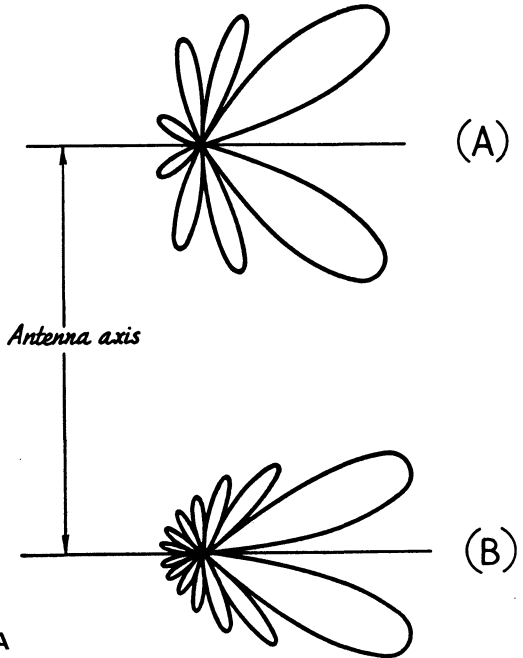
Fig. 5-11 — Typical radiation patterns (cross section of solid figure) for terminated long wires. (A) length two wavelengths, (B) four wavelengths, both for an idealized case in which there is no decrease of current along the wire. In practice, the pattern is somewhat distorted by wire attenuation.
