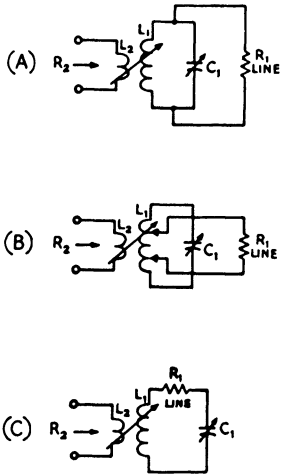
Fig. 3-37 - Circuit arrangements for inductively coupled impedance-matching circuit. A and B use a parallel-tuned coupling tank; B is equivalent to A when the taps are at the ends of L1. The series-tuned circuit at C is useful for very low values of load resistance, R1.
