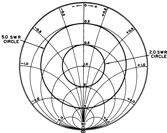
Fig. 3-19 — Smith Chart with SWR circles added.
