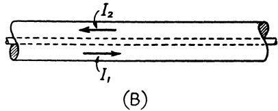
Fig. 3-1 – The two basic types of transmission lines.
