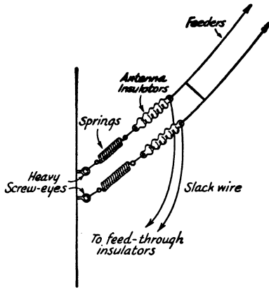
Fig. 13-13 — Anchorage for open-wire line at the station end. The springs are especially desirable if the line is not supported between the antenna and the anchoring point.
