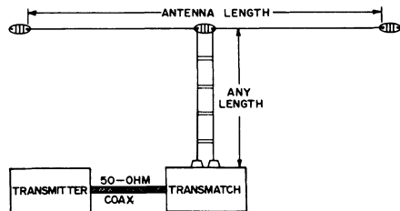
Fig. 6-4 — A center-fed antenna system for multiband use.
