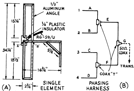
Fig. 11-49 - At A, constructional details of one of the dipole elements of Fig. 11-48. The phasing harness is shown at B.
