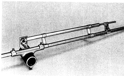
Fig. 11-22 — Gamma matching section using tubular capacitor. The sheet-aluminum clip at the right is moved along the driven element for matching. The small rod can be slid in and out of the 15-inch tube for adjustment of series capacitance. The rod should be about 14 inches long.
