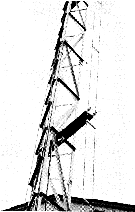
Fig. 13-12 — A board fitted with standoff insulators and clamped to the tower with U bolts keeps open-wire line suitably spaced from a tower. (W4NML.)
