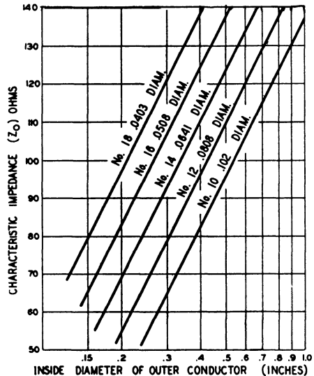
Fig. 3-32 — Characteristic impedance of typical air-insulated coaxial lines.
