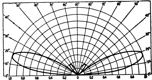
Fig. 4-19 — Vertical pattern broadside to a two-element in-phase array with horizontal elements. This pattern is for a mean height of 3/4 wavelength, i.e., lower element 1/2 wavelength high and upper element one wavelength high. At low wave angles, the horizontal pattern of such an array is the same as for a half-wave dipole.
