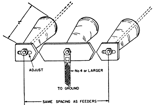
Fig. 13-16 — A simple lightning arrester for open-wire line made from three standoff or feed-through insulators and sections of 1/8 X 1/2-inch brass or copper strap. It should be installed in the line at the point where the line enters the station. The heavy ground lead should be as short and direct as possible. The gap setting should be adjusted to the minimum width that will prohibit arcing when the transmitter is operated.
