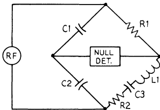
Fig. 17-17 — The basic circuit of the Macro-matcher. In this circuit the bridge is balanced before measurements are made, by setting X_{L1} = X_{C3} .
