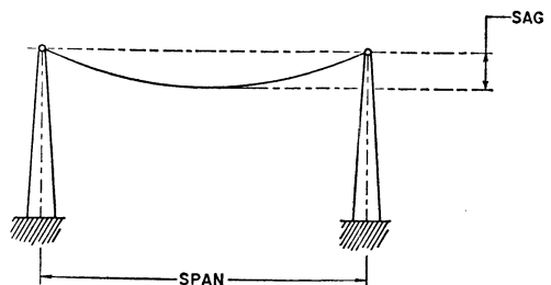
Fig. 13-1 — The span and sag of a long-wire antenna.
