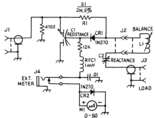
Fig. 17-18 — Schematic diagram of the Macro-matcher. Capacitance is in microfarads; resistance is in ohms, k = 1000. Resistors are 1/2-W 10-percent tolerance unless otherwise indicated.
