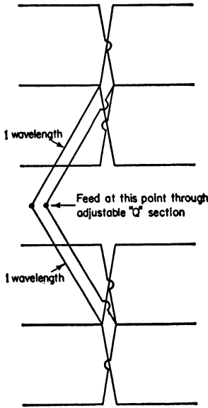
Fig. 11-34 — Method of feeding the driven elements of a 24-element array. Phasing lines may be open-wire line with 1/2 to 1 inch spacing between conductors.
