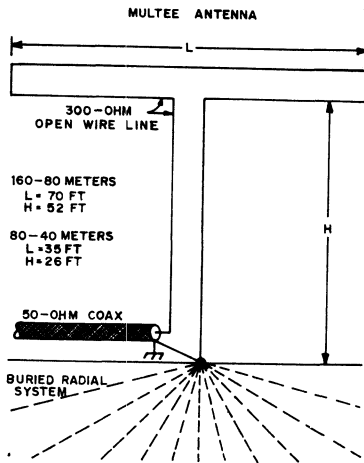
Fig. 16-15 — Two-band operation in limited space may be obtained with the multitee antenna. The feed-line portion should remain as vertical as possible, as it does the radiating on the lower frequency band.
