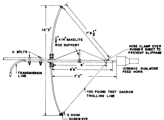
Fig. 12-11 - Side view of the stressed parabolic dish.
