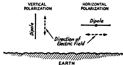
Fig. 2-11 — Vertical and horizontal polarization of a dipole. The direction of polarization is the direction of the electric field with respect to earth.
