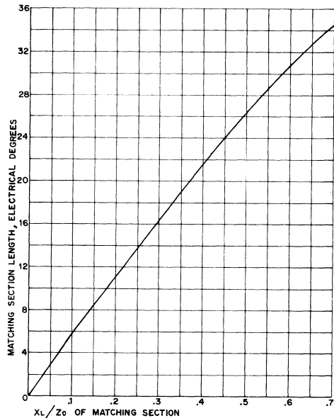
Fig. 3-72 — Inductive reactance (normalized to Z_0 of matching section), scale at bottom, versus required matching-section length, scale at left. To determine the length in wavelengths, divide the number of electrical degrees by 360. For open-wire line, a velocity factor of 97.5% should be taken into account when determining the electrical length.
