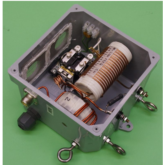
Fig 6 – Ventilated Enclosure
